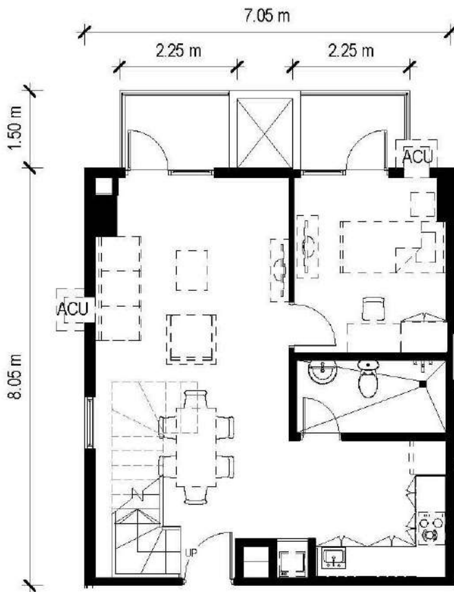
KEYPLAN - 29TH FLOOR
