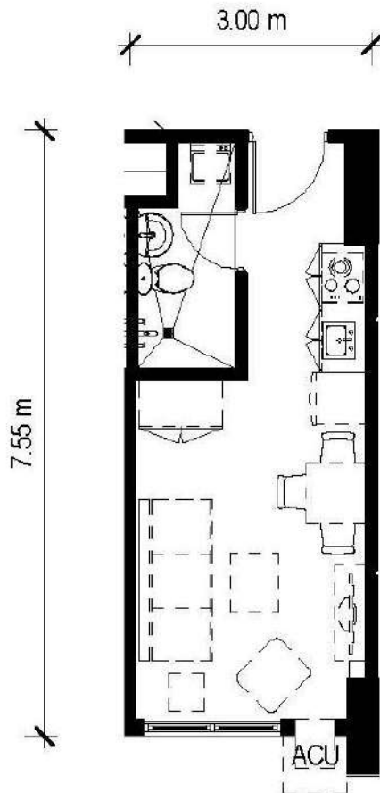
KEYPLAN - 5TH TO 28TH FLOOR (TYPICAL)
