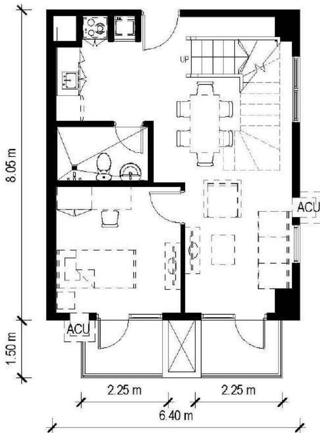
KEYPLAN - 29TH FLOOR
