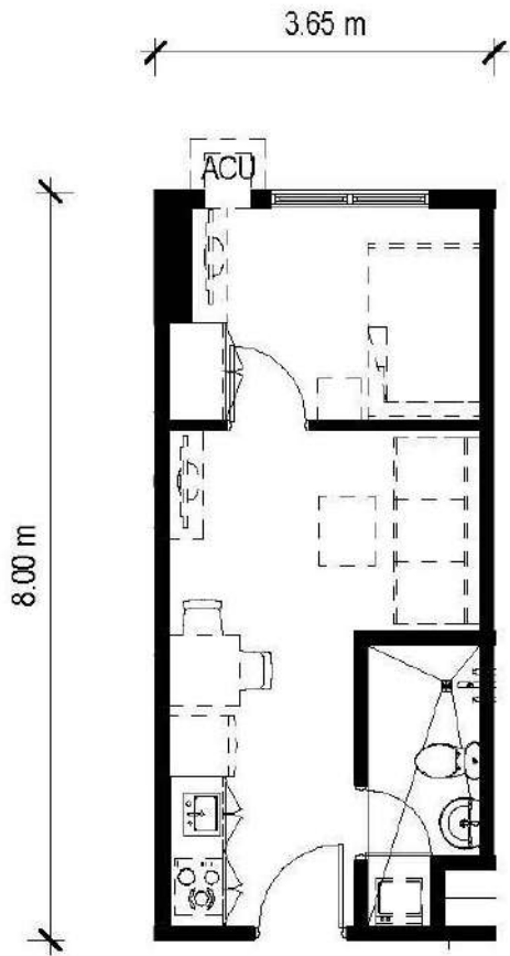
KEYPLAN - 5TH TO 28TH FLOOR (TYPICAL)
